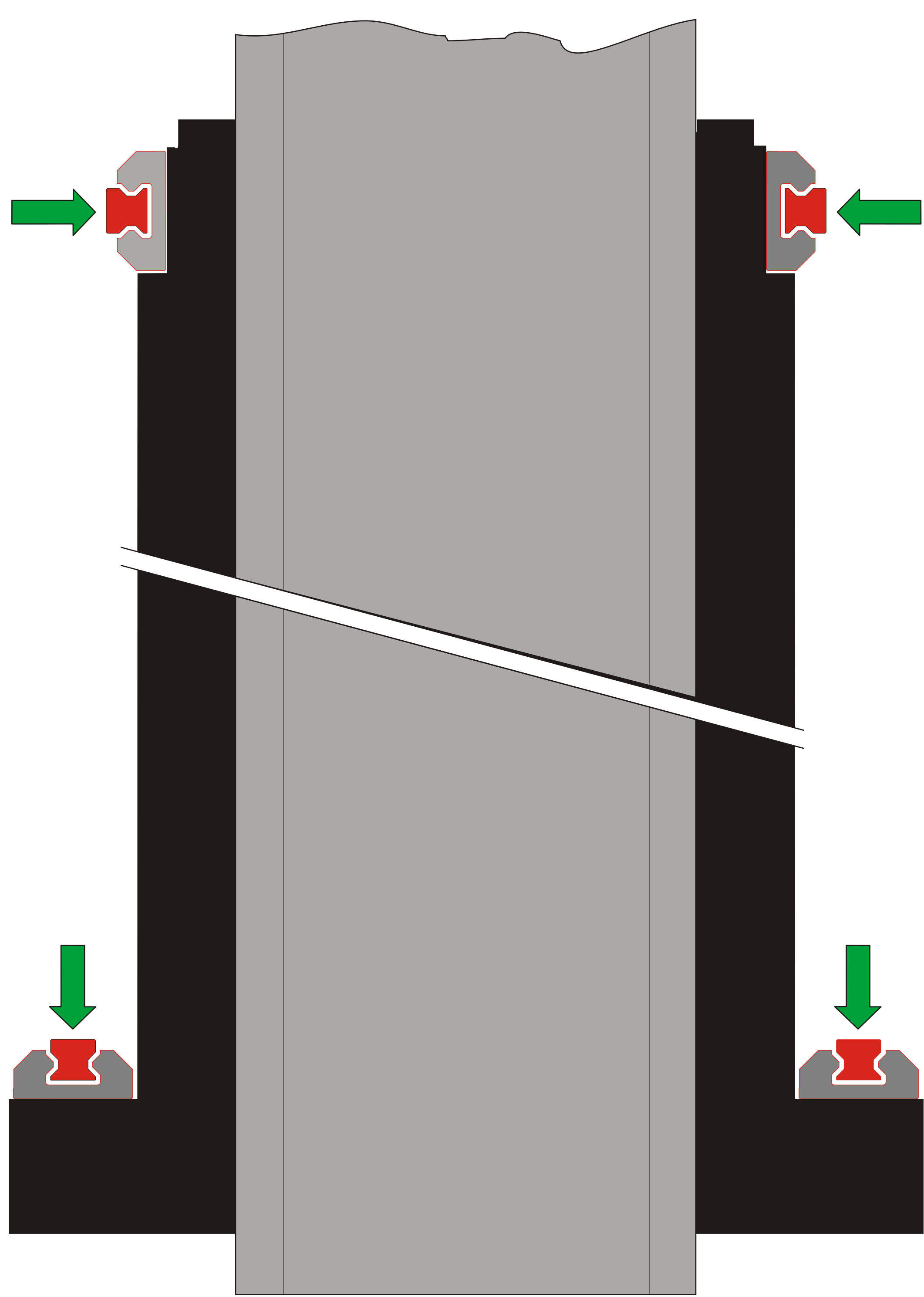
MOVIMENTO VERTICALE VERTICAL TRAVEL
